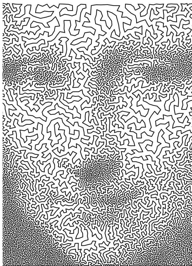
Figure 4. This continuous line drawing of Leonardo DaVinci's "Mona Lisa" uses 10,000 cities and is topologically equivalent to a circle.
